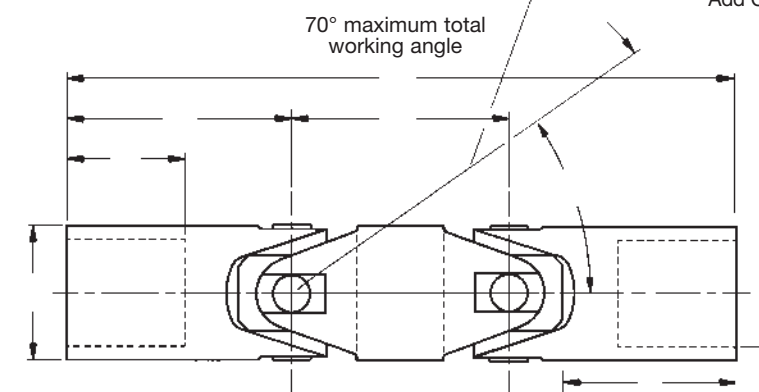
Double - Uncovered
