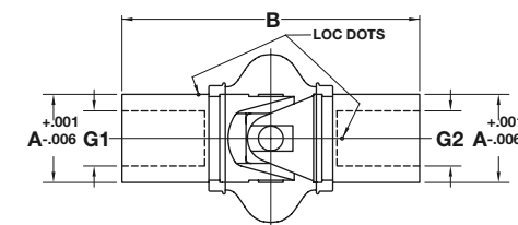
Style S
