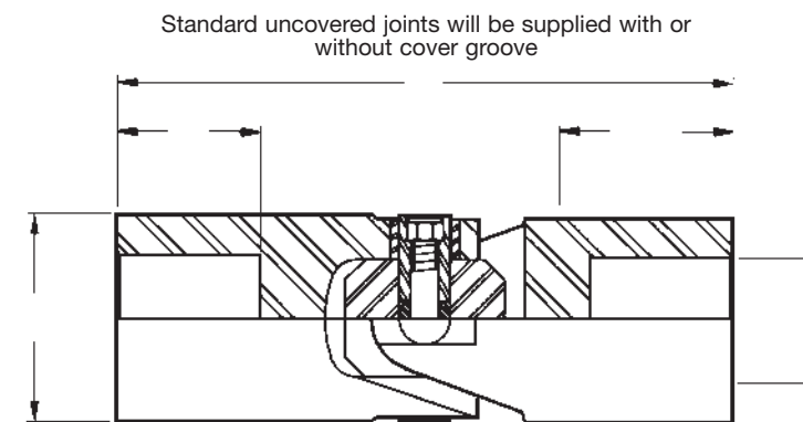
400 Series - Uncovered
