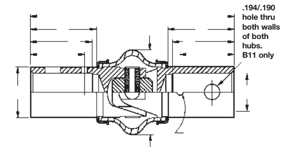
MS 271 Series
