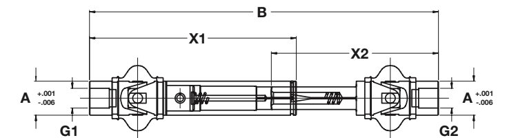
Style X
